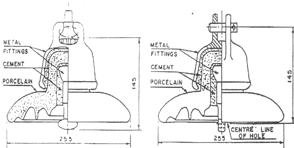
FIG-2A BALL AND SOCKET TYPE.
